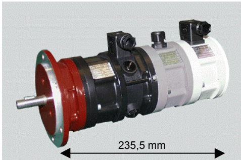
DC tachogenerator, optical encoder, centrifugal switch
